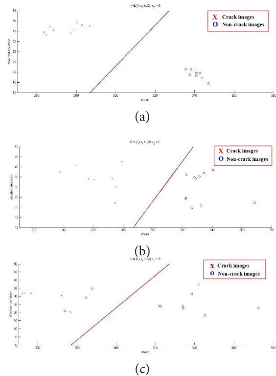
Figure 10. Scatter plot of tested images by quality, (a) good, (b) medium, (c) low.
