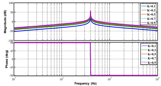
Figure 6. Bode of the Controller by changing the value K (resonant gain).
