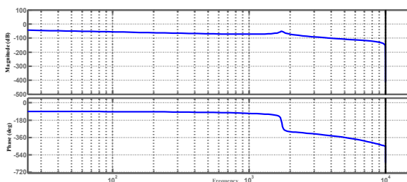
Figure 5. Bode of the discrete system PI controller.
