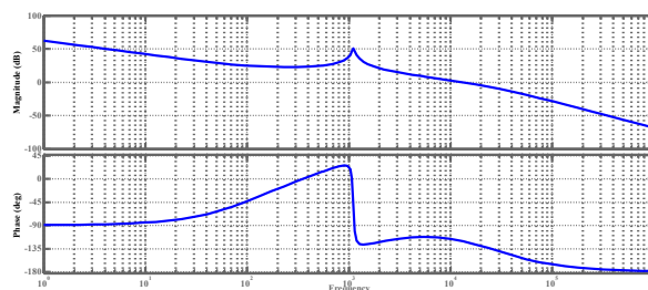
Figure 4. Bode of continuous of the system with PID controller.
