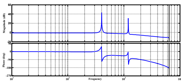
Figure 9. Bode of the system using 5th harmonic PR controller.
