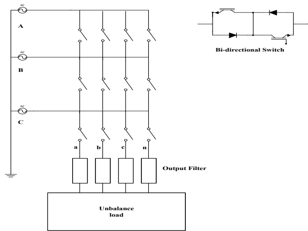
Figure 1. Three Phase Matrix Converter diagram.
