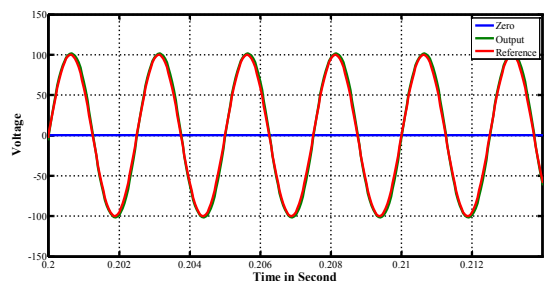
Figure 11. Output sine wave after 0.2 second.
