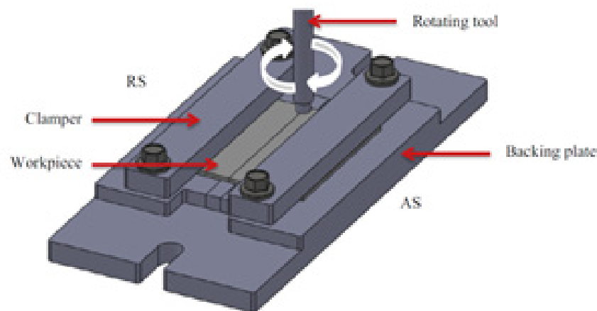
Figure 1. Assembly of jig and fixture with rotating tool.
