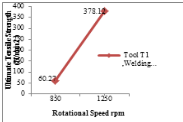
Figure 5. UTS at Constant Welding Speed of 40mm/min.
