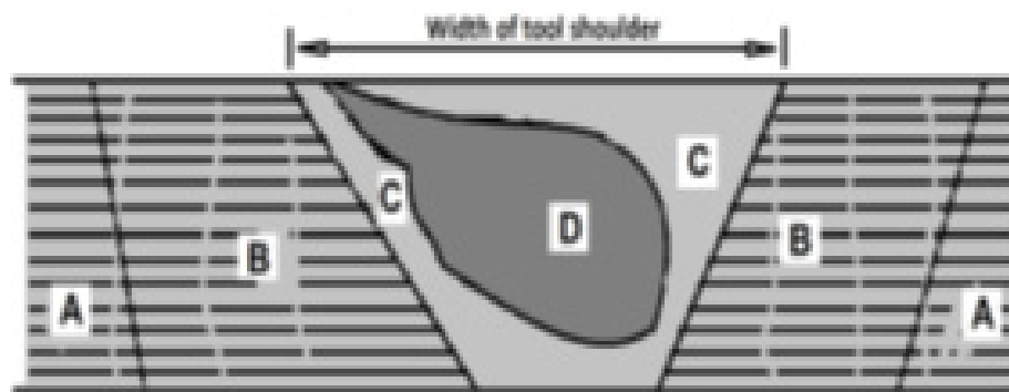
Figure 1. Various microstructural zones in the transverse cross section of FSWed metal plates.
