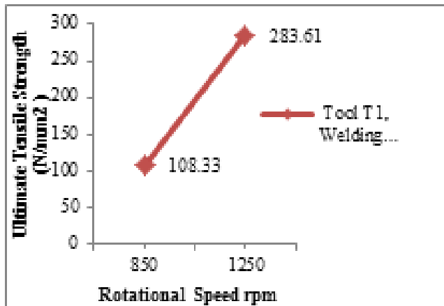
Figure 4. UTS at Constant Welding speed 30mm/min.
