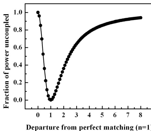
Figure 5. Response of uncoupled power to departure from perfect matching. At perfect matching condition ( n = \omega_r / \omega_m = 1 ), the uncoupled power is zero. The uncoupled power increases with increase of departure in both the direction. With n = 6 or n = \frac{1}{6} the uncoupled power drops to 90 % of the peak value.
