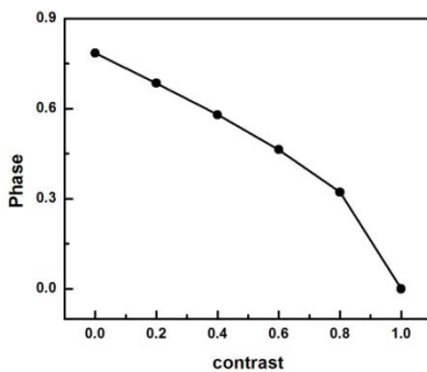
Figure 1. Variation of phase with contrast. More the intensities of individual beams are unbalanced, more is the departure of contrast from unity leading to a gradual enhancement of wave front slope at the retina.
