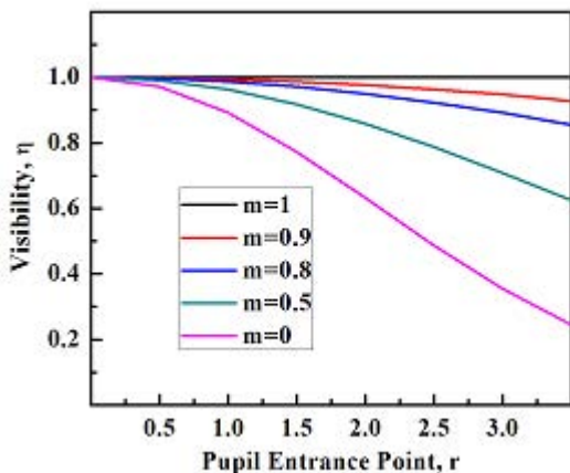
Figure 3. Variation of visibility with pupil entry point for different departures. Nil departure ( m = 1 ) is independent of pupil entry point, other departures ( m \neq 1 ) are pupil entry point dependent with maximum departure ( m = 0 ) showing maximum response in the form of more visibility loss.
