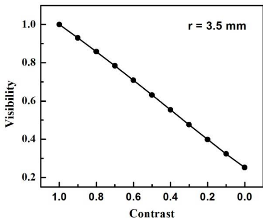
Figure 4. Variation of visibility with contrast. Gradual enhancement of the departure from zero to maximum (i.e., m = 1 to m = 0 ) the visibility drops to 24 % of its peak value.
