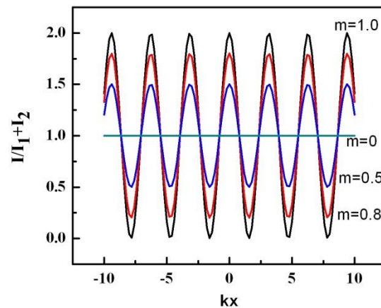
Figure 2. The intensity distribution for nil departure from unit contrast ( m = 1 ), maximum departure for m = 0 , and intermediate departures for m = 0.5 and m = 0.8 .
