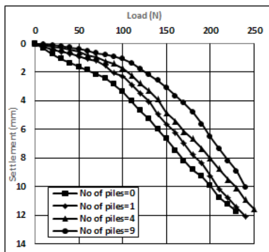
Figure 5. Load vs. settlement curve with raft size 200x200x10 mm (rigid).
