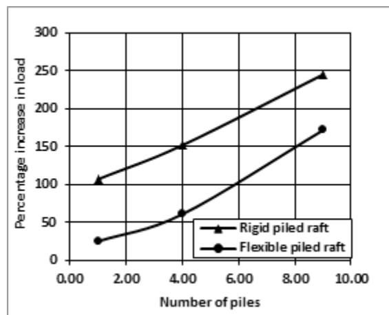
Figure 7. Percentage increase in load carrying capacity of piled raft system with different numbers of piles at settlements of 1 mm for both rigid and flexible rafts.
