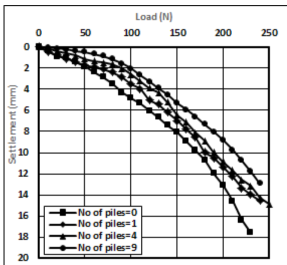
Figure 4. Load vs. settlement curve with raft size 200x200x2 mm (flexible).
