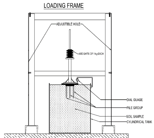
Figure 3. Pile raft model with loading arrangement.
