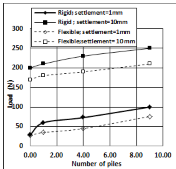
Figure 6. Load carrying capacity of piled raft system with different numbers of piles at settlements of 1mm and 10mm for both rigid and flexible rafts.
